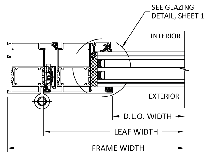
C 4 HORIZONTAL SECTION JAMB DETAIL - OUTSWING DOOR
