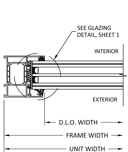
A 4 HORIZONTAL SECTION JAMB DETAIL - SIDELITE
